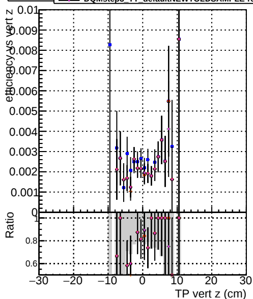
Efficiency Configuration ~0.85 DOMstep3 TT cktPixelLess ~0.75 DOMstep3 TT default-rlf ~0.65 DOMstep3 TT defaultNEWTOLDSAMPLE-rlf
