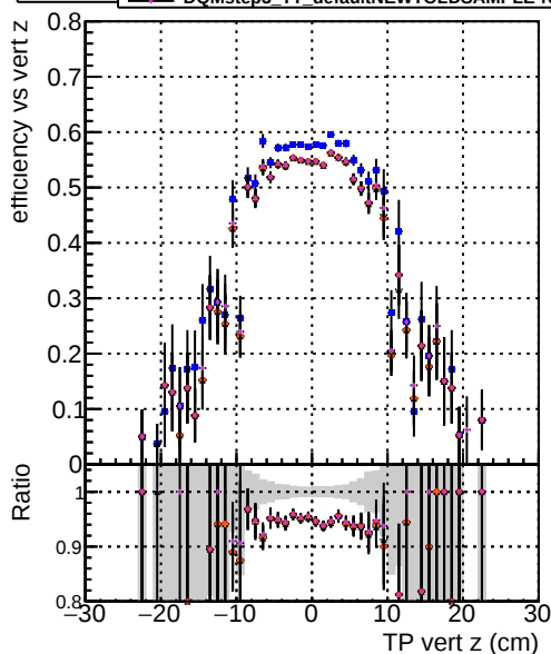
Efficiency Model Dataset Method ~0.85 DOMstep3 TT ckptPixelLess ~0.80 DOMstep3 TT default-relf ~0.75 DOMstep3 TT defaultNEWTOLDSAMPLE-relf
