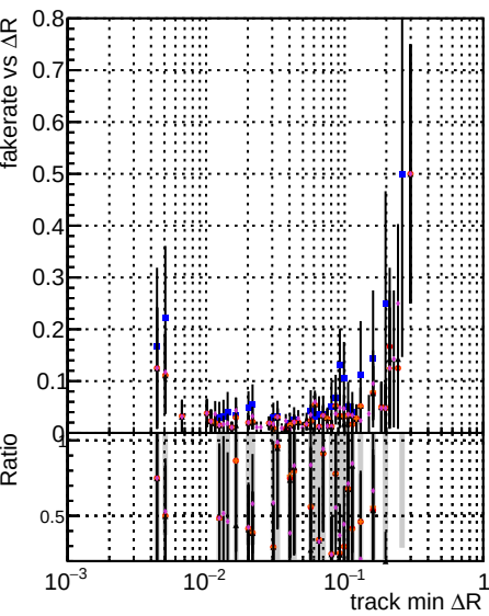
Fake rate vs ΔR(track, jet) for various models: DOM, Meten3, TT, GKE, default, relf, NEWTOLD, SAMPLE-relf
