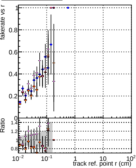
Fake rate vs v Legend: DOM, Metep3, TTK, GKE, default, cell-less, NEWTOLDSAMPLE-reif
