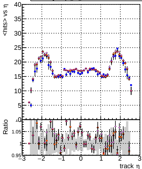
mean hits vs \eta Legend for mean hits vs \eta : DOMstep3 TT CKF DOMstep3 TT default DOMstep3 TT ckPixelLess DOMstep3 TT default-ref DOMstep3 TT defaultNEWTOLDSAMPLE-ref
