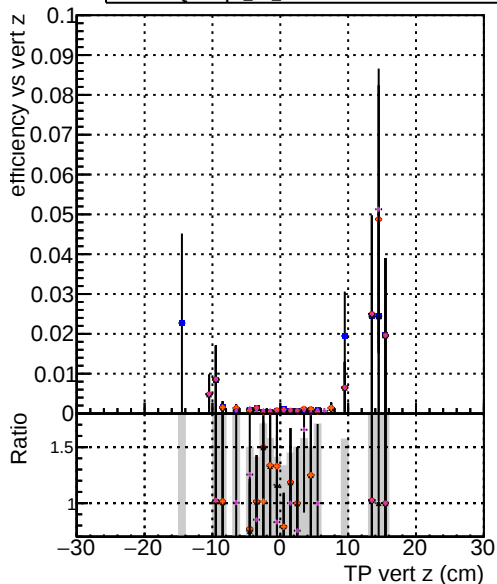
Efficiency Series Configuration ~0.85 DOMstep3 TT ckfPixelLess ~0.75 DOMstep3 TT default-rlf ~0.65 DOMstep3 TT defaultNEWTOLDSAMPLE-rlf
