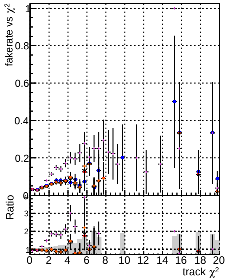
Fake rate vs. track \chi^2
