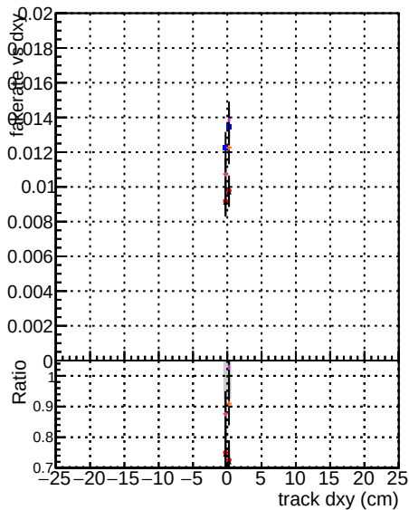
Fake rate vs d Duplicates rate vs d Pileup rate vs d Fake rate vs dz Duplicates rate vs dz Pileup rate vs dz
