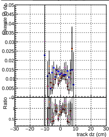
Fake rate vs d Duplicates rate vs d Pileup rate vs d Fake rate vs dz Duplicates rate vs dz Pileup rate vs dz
