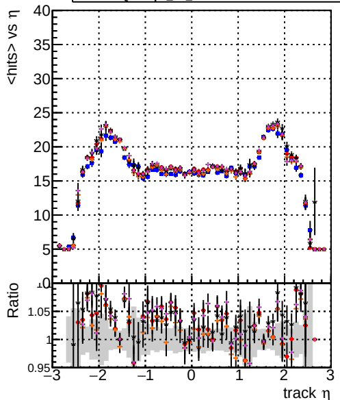
mean hit DOMstep3 TT CKF DOMstep3 TT ckfPixelLess DOMstep3 TT default-ref DOMstep3 TT default-NEWTOLDSAMPLE-ref
