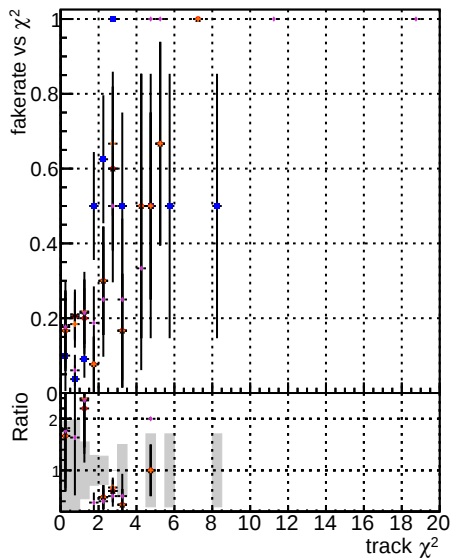
Fake rate vs. DQM steps3 TT default NEW TOLD SAMPLE relf
