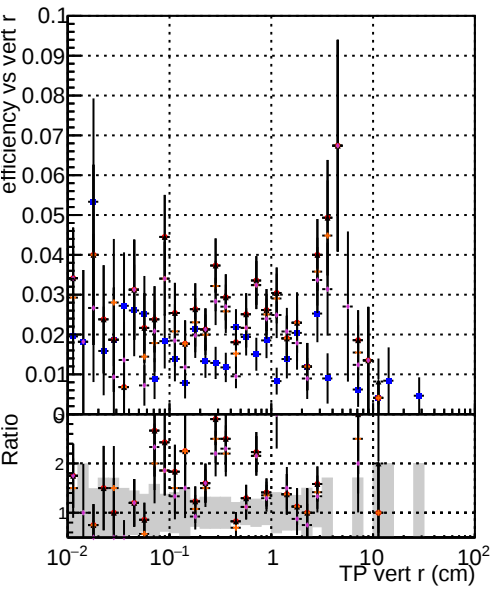
Efficiency vs vertpos DOMstep3 CKF DOMstep3 default DOMstep3 ckPixelLess DOMstep3 default-relu DOMstep3 defaultNEWTOLDSAMPLE-relu
