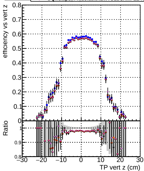
Efficiency Series Method Configuration ~0.85 Black DOMstep3 TT cktPixelLess ~0.75 Orange DOMstep3 TT default-rlf ~0.65 Purple DOMstep3 TT defaultNEWTOLDSAMPLE-rlf
