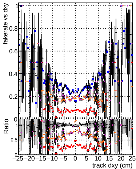
Fake rate vs d Duplicates rate vs dxy Pileup rate vs dxy Ratio vs track dxy (cm)
