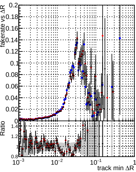
Legend: DOMstep3_SoftQCD_CKF (blue line with dots), DOMstep3_SoftQCD_default (red line with dots), DOMstep3_SoftQCD_ckfPixelLess (black line with dots)
