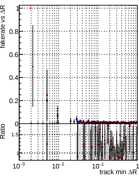
Fake rate vs \Delta R(\text{track, jet}) Legend: DOMstep3_SoftQCD_CKF (black line with dots) DOMstep3_SoftQCD_default (red line with dots) DOMstep3_SoftQCD_ckfPileLess (blue line with dots)
