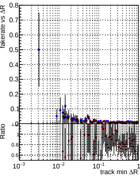
Legend: DOMstep3_SoftQCD_CKF (blue circles) DOMstep3_SoftQCD_default (red circles) DOMstep3_SoftQCD_ckfPixelLess (black circles)
