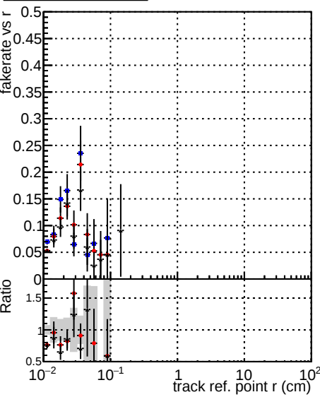
Fake rate vs verpos Legend: DOMstep3_SoftQCD_CKF (blue dots) DOMstep3_SoftQCD_default (red dots) DOMstep3_SoftQCD_ckfPixelLess (black dots)
