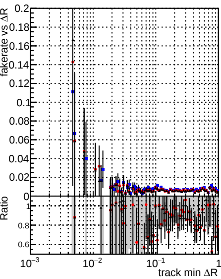
Fake rate vs ΔR(track, jet) Legend: DOMstep3_SoftQCD_CKF (blue dots) DOMstep3_SoftQCD_default (red dots) DOMstep3_SoftQCD_ckfPileLess (black dots)
