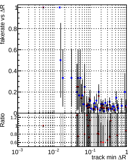
Fake rate vs \Delta R(\text{track, jet}) Legend: DOMstep3_SoftQCD_CKF (blue squares) DOMstep3_SoftQCD_default (red circles) DOMstep3_SoftQCD_ckfPileLess (black triangles)
