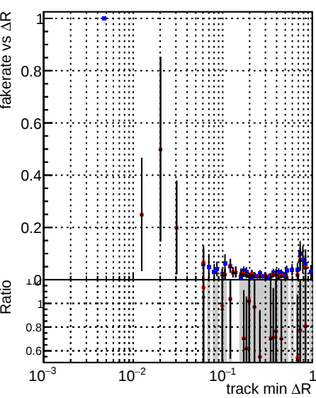
Fake rate vs \Delta R(\text{track, jet}) Legend: DQMstep3_SoftQCD_CKF (blue dots) DQMstep3_SoftQCD_default (red dots) DQMstep3_SoftQCD_ckfPileLess (black dots)
