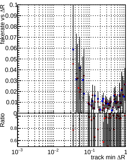
Fake rate vs \Delta R(\text{track}, \text{jet}) Legend: DOMstep3_SoftQCD_CKF (blue dots) DOMstep3_SoftQCD_default (red dots) DOMstep3_SoftQCD_ckfPileLess (black dots)
