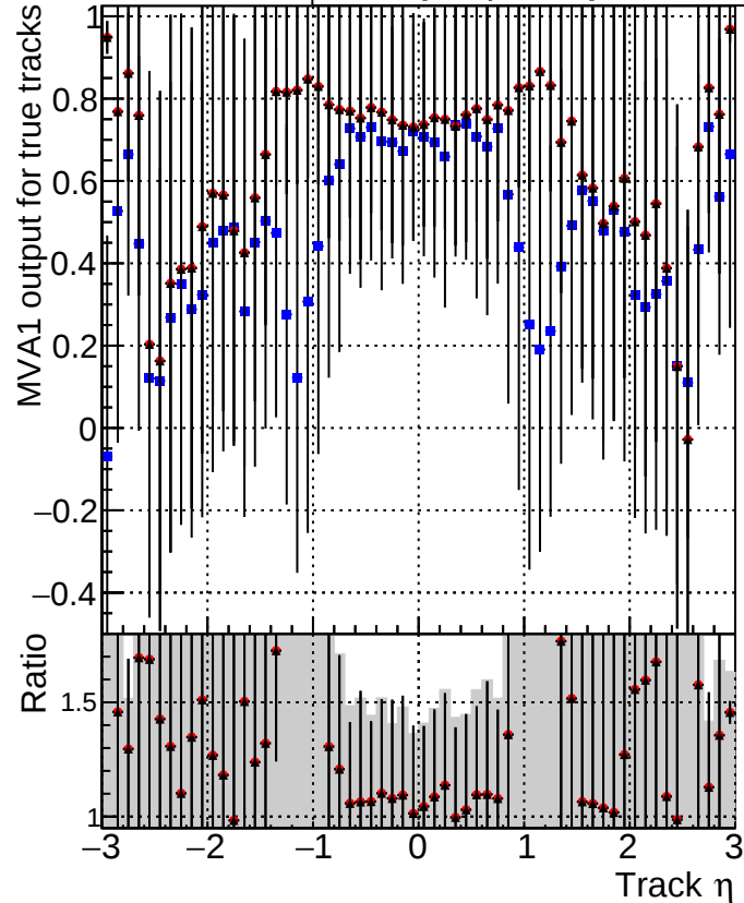
MVA1 of associated tracks (recoToSim) vs. track \eta Legend: ■ DQMstep3_SoftQCD_CKF ● DQMstep3_SoftQCD_default ▲ DQMstep3_SoftQCD_ckfPixelLess
