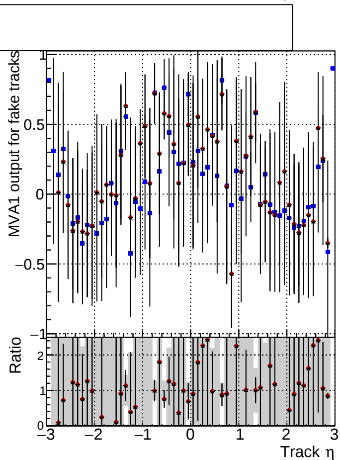
MVA1 of associated tracks (recoToSim) vs. track \eta Legend: ■ DQMstep3_SoftQCD_CKF ● DQMstep3_SoftQCD_default ▲ DQMstep3_SoftQCD_ckfPixelLess
