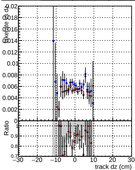
— DOMstep3 SoftOCB-CKF — DOMstep3 SoftOCB-CKF d default — DOMstep3 SoftOCB-CKF PixelLess
