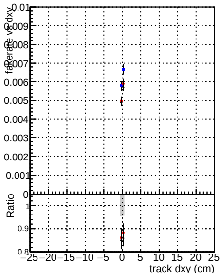
— DOMstep3 SoftOCB-CKF — DOMstep3 SoftOCB-CKF d default — DOMstep3 SoftOCB-CKF PixelLess
