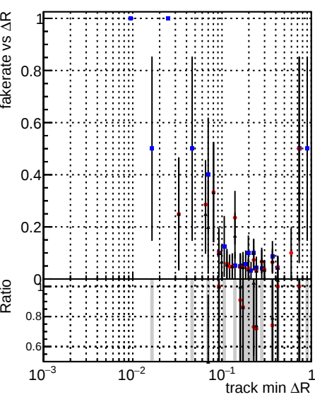
Fake rate vs \Delta R(\text{track, jet}) Legend: DQMstep3_SoftQCD_CKF (blue squares) DQMstep3_SoftQCD_default (red circles) DQMstep3_SoftQCD_ckfPileLess (black circles with error bars)
