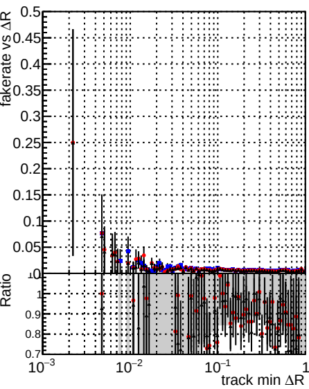
Legend: DOMstep3_SoftQCD_CKF (black line with blue dots), DOMstep3_SoftQCD_default (red line with red dots), DOMstep3_SoftQCD_ckfPileLess (black line with black dots)
