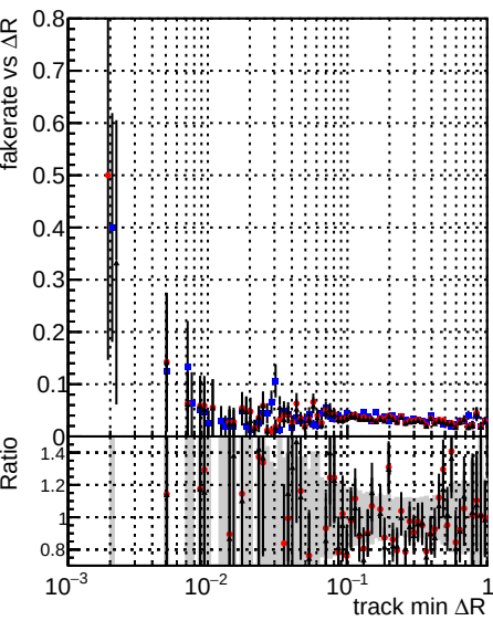
Fake rate vs \Delta R(\text{track, jet}) DOMstep3_SoftQCD_CKF DOMstep3_SoftQCD_default DOMstep3_SoftQCD_ckfPileLess
