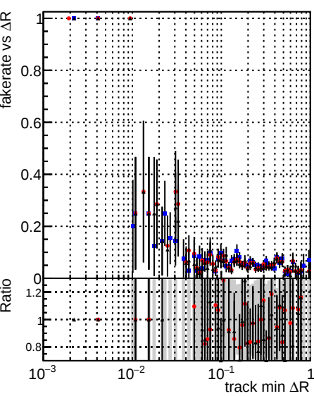
Legend: DQMstep3_SoftQCD_CKF (black line with blue dots), DQMstep3_SoftQCD_default (red line with red dots), DQMstep3_SoftQCD_ckfPixelLess (black line with black dots)
