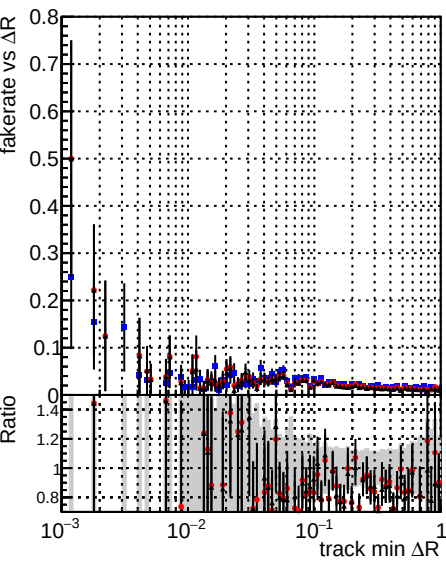
Fake rate vs \Delta R(\text{track, jet}) Legend: DOMstep3_SoftQCD_CKF (blue squares) DOMstep3_SoftQCD_default (red circles) DOMstep3_SoftQCD_ckfPixelLess (black triangles)
