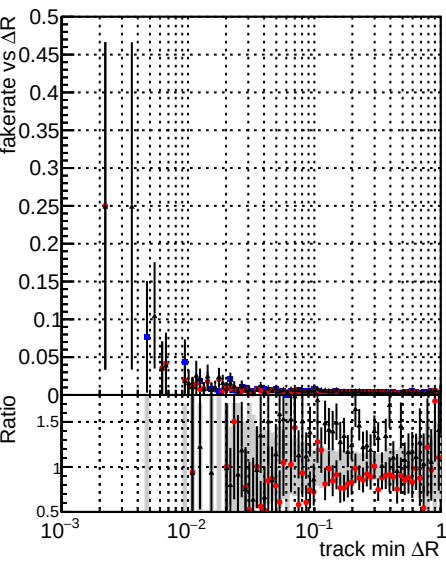
Legend: DOMstep3 SoftQCD CKF (black line), DOMstep3 SoftQCD default (red line), DOMstep3 SoftQCD defaultNEWT (blue line)
