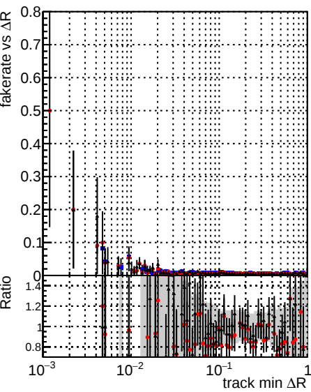
Legend: DOMstep3_SoftQCD_CKF (blue circles), DOMstep3_SoftQCD_default (red circles), DOMstep3_SoftQCD_defaultNEWT (black circles)
