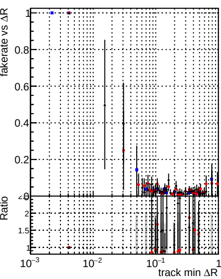
Legend: DQMstep3_SoftQCD_CKF (black line with blue dots), DQMstep3_SoftQCD_default (red line with dots), DQMstep3_SoftQCD_defaultNEWT (black line with dots)
