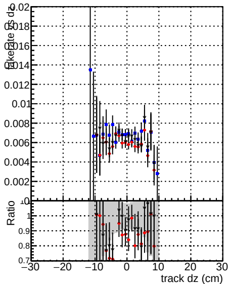
Fake rate vs dz DOMstep3 SoftQCD CKF DOMstep3 SoftQCD default DOMstep3 SoftQCD defaultNEWTT
