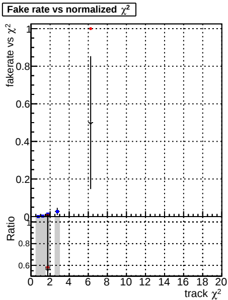
Fake rate vs. \chi^2 Legend: DOMstep3 SoftOCD-CKF DOMstep3 SoftOCD-default DOMstep3 SoftOCD-NEWT
