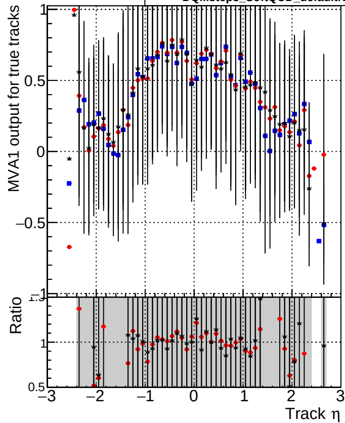
MVA1 of associated tracks (recoToSim) vs. track \eta Legend: DQMstep3_SoftQCD_CKF (blue squares) DQMstep3_SoftQCD_default (red circles) DQMstep3_SoftQCD_defaultNEWT (black stars)
