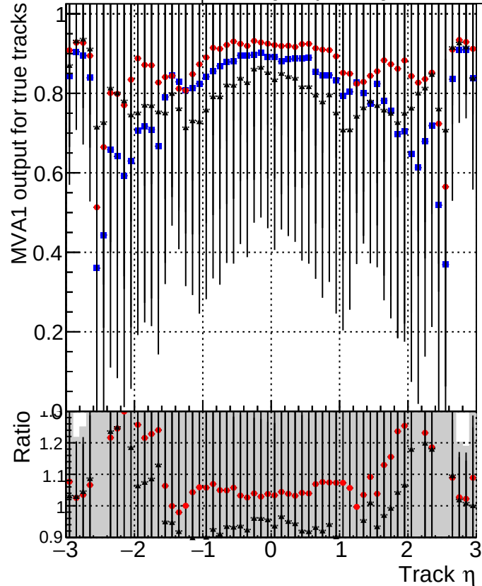
MVA1 of associated tracks (recoToSim) vs. track \eta Legend: DQMstep3_SoftQCD_CKF (blue squares) DQMstep3_SoftQCD_default (red diamonds) DQMstep3_SoftQCD_defaultNEWT (black stars)
