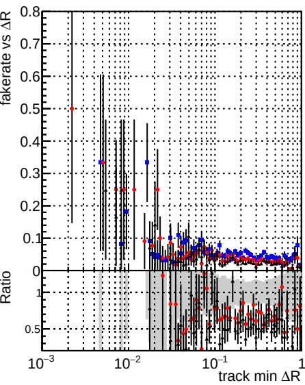
Fake rate vs \Delta R(\text{track}, \text{jet}) Legend: DOMstep3 SoftQCD CKF (black line with blue dots) DOMstep3 SoftQCD default (red line with red dots) DOMstep3 SoftQCD defaultNEWT (black line with black dots)
