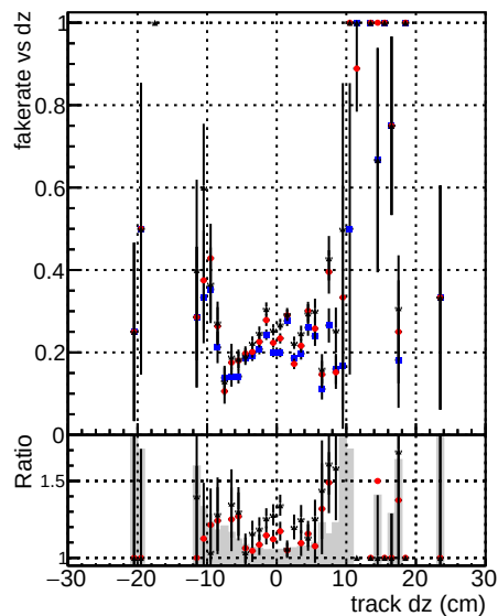
Fake rate vs d DOMstep3 SoftOCB-CKF DOMstep3 SoftOCB-default DOMstep3 SoftOCB-defaultNEW2
