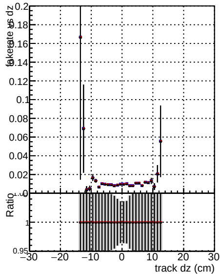
Fake rate vs dz DOMstep3 SoftQCD CKF DOMstep3 SoftQCD default DOMstep3 SoftQCD defaultNEW2
