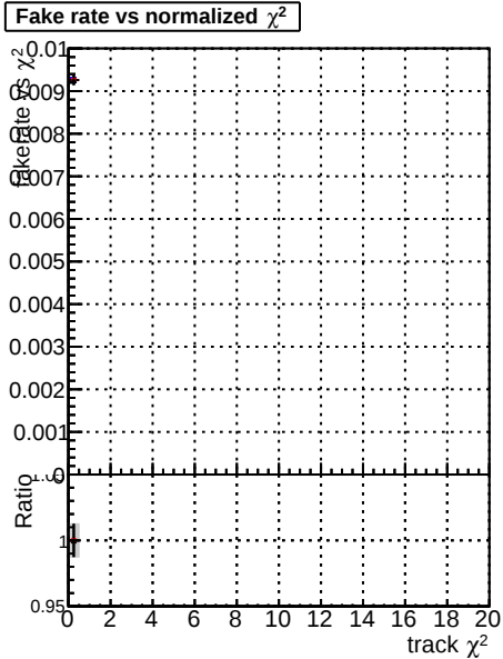
Fake rate vs. DOMstep3 SoftQCD CKF, DOMstep3 SoftQCD default, DOMstep3 SoftQCD defaultNEWT2
