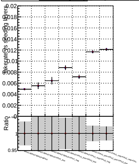
Fake rate vs. DOMstep3 SoftQCD CKF, DOMstep3 SoftQCD default, DOMstep3 SoftQCD defaultNEWT2
