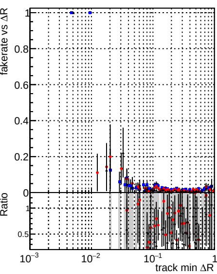
Fake rate vs ΔR(track, jet) DOMstep3 SoftQCD CKF DOMstep3 SoftQCD default DOMstep3 SoftQCD defaultNEW2
