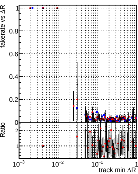
Legend: DQMstep3_SoftQCD_CKF (black line with blue dots), DQMstep3_SoftQCD_default (red line with red dots), DQMstep3_SoftQCD_defaultNEWT2 (black line with black dots)
