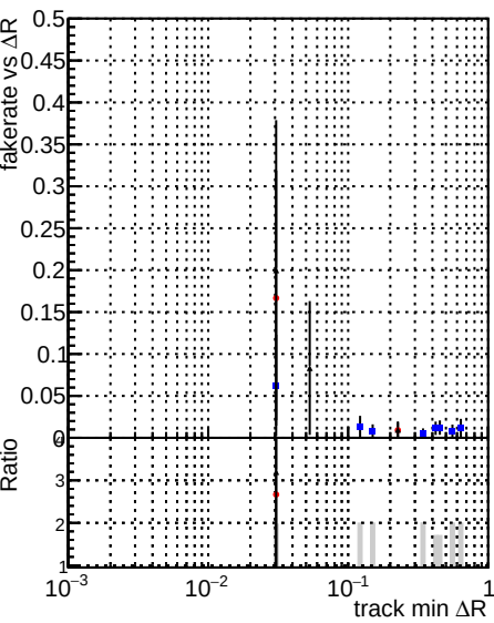
Legend: DOMstep3_SoftQCD_CKF (blue dots), DOMstep3_SoftQCD_default (red dots), DOMstep3_SoftQCD_defaultNEWT2 (black dots)
