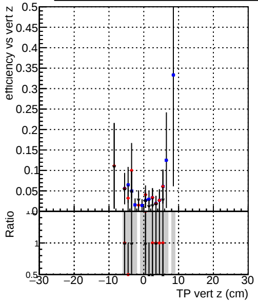
Efficiency vs TP vertex z (z)
