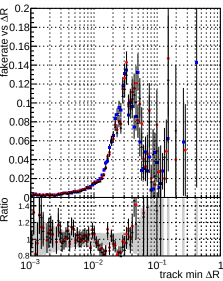
Fake rate vs \Delta R(\text{track, jet}) Legend: DOMstep3 SoftQCD CKF DOMstep3 SoftQCD default DOMstep3 SoftQCD defaultNEWT3
