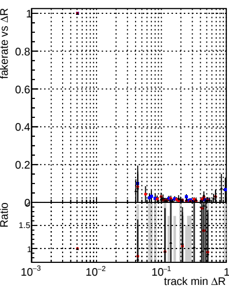
Legend: DOMstep3_SoftQCD_CKF (grey line with blue dots), DOMstep3_SoftQCD_default (red line with red dots), DOMstep3_SoftQCD_defaultNEWT3 (black line with black dots)
