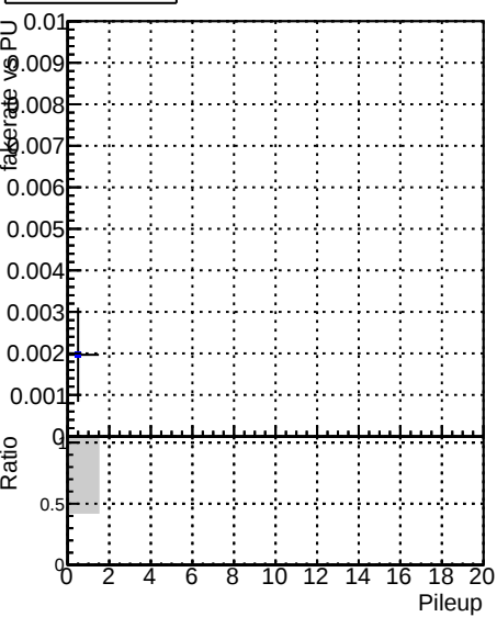
Fake rate vs Pileup
