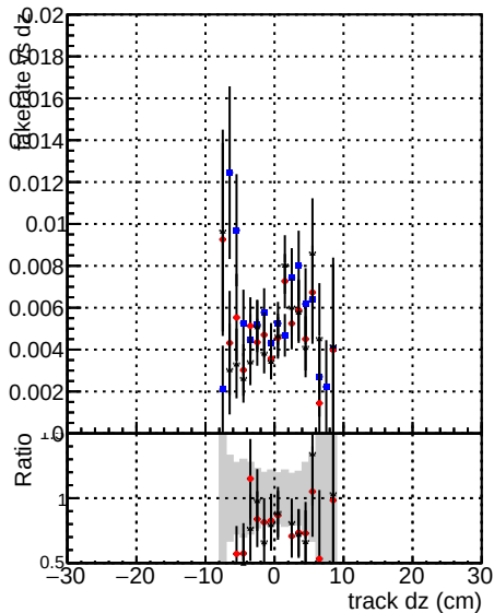
Fake rate vs dz DOMstep3 SoftQCD CKF DOMstep3 SoftQCD default DOMstep3 SoftQCD defaultNEWT3
