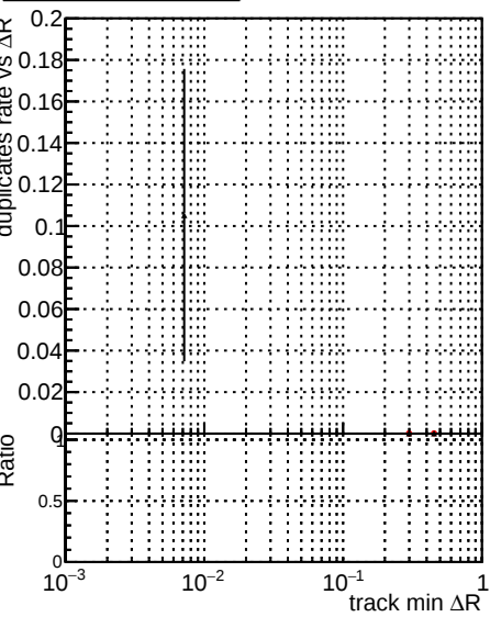
Legend: DOMstep3_SoftQCD_CKF (black line with blue dots), DOMstep3_SoftQCD_default (black line with red dots), DOMstep3_SoftQCD_defaultNEWT3 (black line with black dots)
