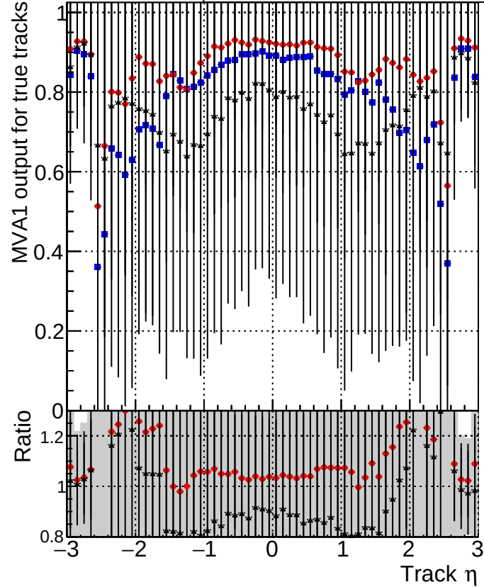
MVA1 of associated tracks (recoToSim) vs. track \eta Legend: DQMstep3_SoftQCD_CKF (blue squares) DQMstep3_SoftQCD_default (red diamonds) DQMstep3_SoftQCD_defaultNEWT3 (black stars)
