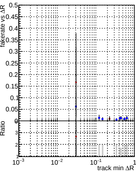
Legend: DOMstep3_SoftQCD_CKF (blue dots), DOMstep3_SoftQCD_default (red dots), DOMstep3_SoftQCD_defaultNEWT20 (black dots)
